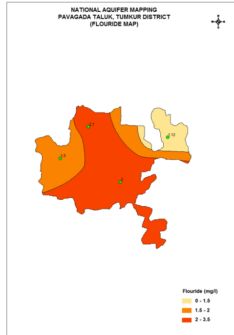
Figure-18: Distribution of Fluoride
