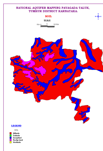
Figure-5: Soil map
