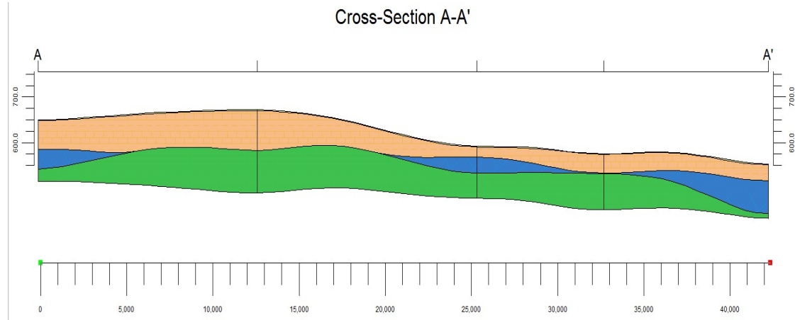
Figure-14B. Aquifer disposition 3 -D Diagram Cross section East-West
