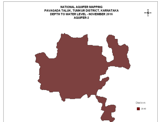
Figure-9: Post monsoon DTW map Aquifer II
