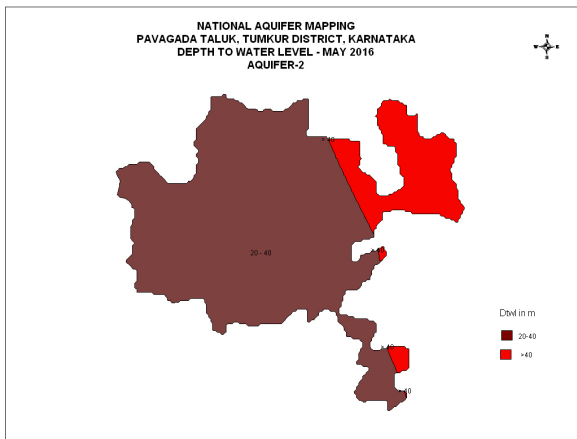
Figure-8: Pre monsoon DTW Map Aquifer II
