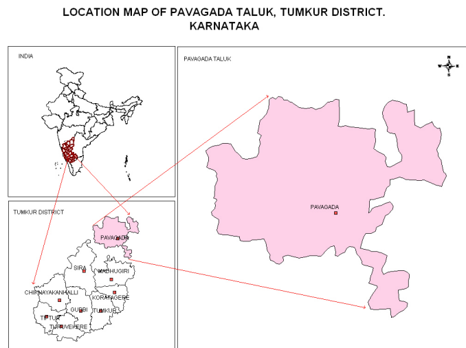
Figure-1: Location Map of Pavagada Taluk, Tumkur district
