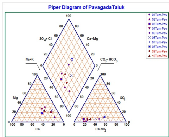
Figure-19 Chemical analysis Plot on Piper Diagram
