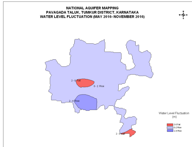
Figure-10 Water Level Fluctuation map Aquifer I
