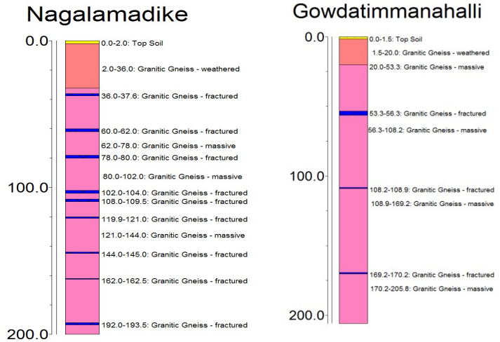
Fig-12 Log diagram of Exploratory wells
