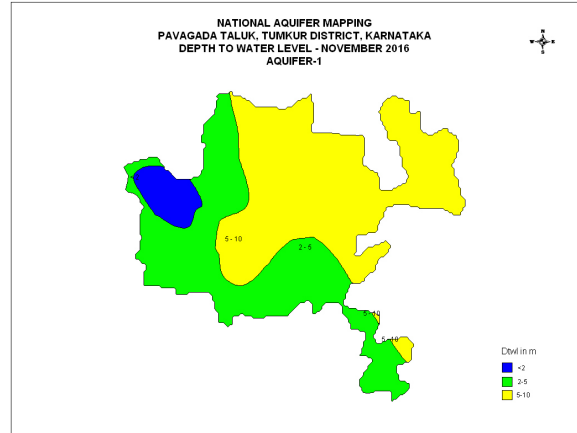
Fig-7 :Post monsoon DTW map Aquifer-I
