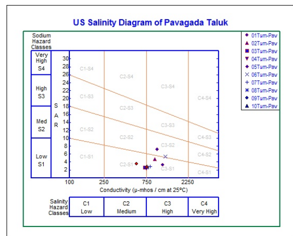
Figure-20 U.S. Salinity diagram
