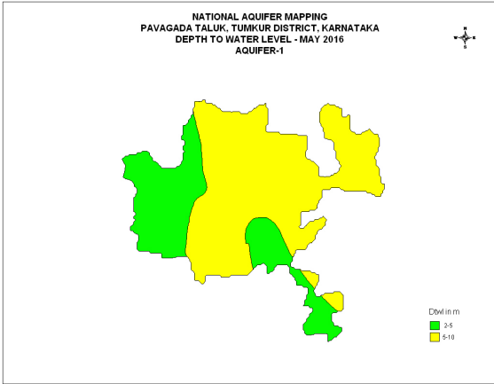
Fig-6: Pre monsoon DTW Map Aquifer I
