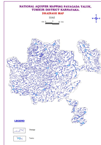
Figure-3 Drainage map
