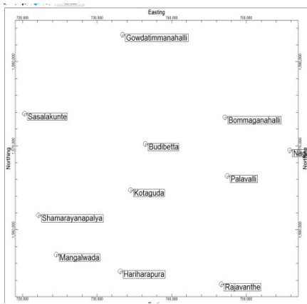
Fig-11 Location map of EW/OW
