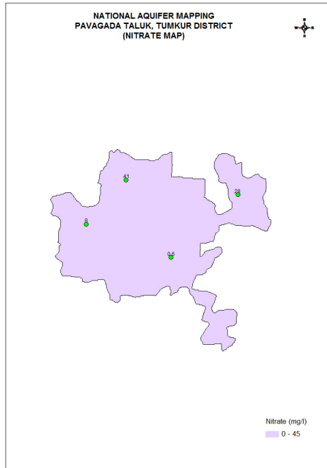
Figure-17: Distribution of Nitrate
