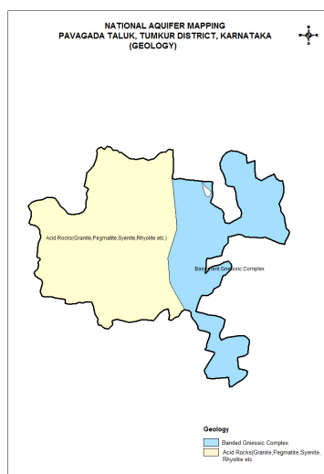
Figure-4: Geology map
